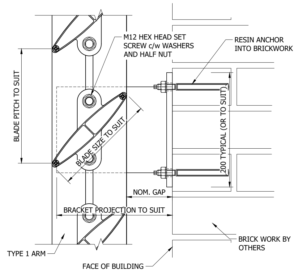
CLIMATE FACADE (TYPE 1 ARM) TO BRICK WORK FIXING DETAIL
