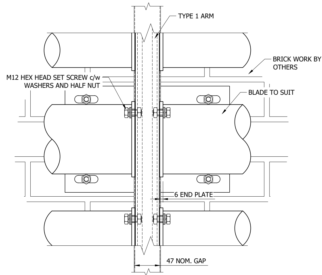
CLIMATE FACADE (TYPE 1 ARM) TO BRICK WORK FIXING DETAIL
